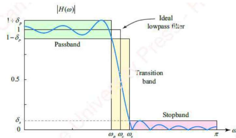
Figure 7.2 Specification of filter characteristics
