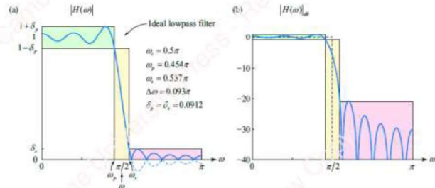
Figure 7.9 Frequency response of magnitude of an FIR filter on linear and log (dB) scales
