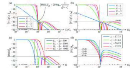
Figure 8.10 Dependence of the inverse Chebyshev filter on parameters N , \Omega_c , and \epsilon_s .
