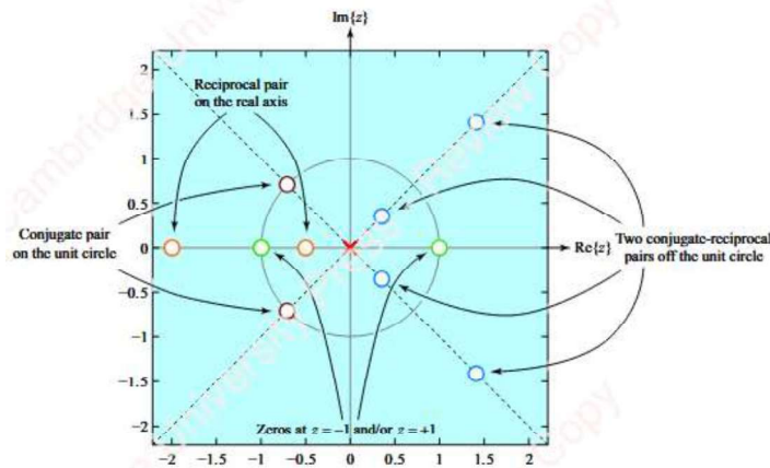
Figure 4.15 Position of zeros for linear-phase FIR systems
